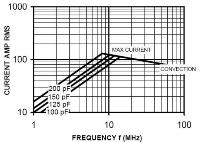
CONTINUOUS RMS AMPERES VS FREQUENCY (AT 18 KV PEAK WORKING VOLTAGE)
