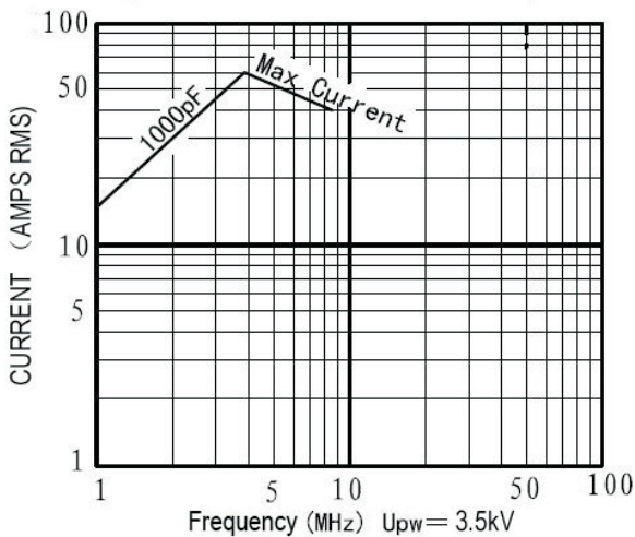
CONTINUOUS RMS AMPERES vs FREQUENCY (at 3.5kV PEAK WORKING VOLTAGE)
