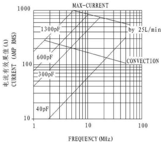
CONTINUOUS RMS AMPERES vs FREQUENCY (at 35KV PEAK WORKING VOLTAGE) 持续有效电流和频率曲线 (在35KV峰值电压工作时测得)
