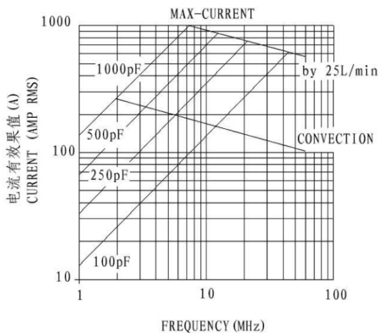
CONTINUOUS RMS AMPERES vs FREQUENCY (at 35KV PEAK WORKING VOLTAGE) 持续有效电流和频率曲线 (在35KV峰值电压工作时测得)
